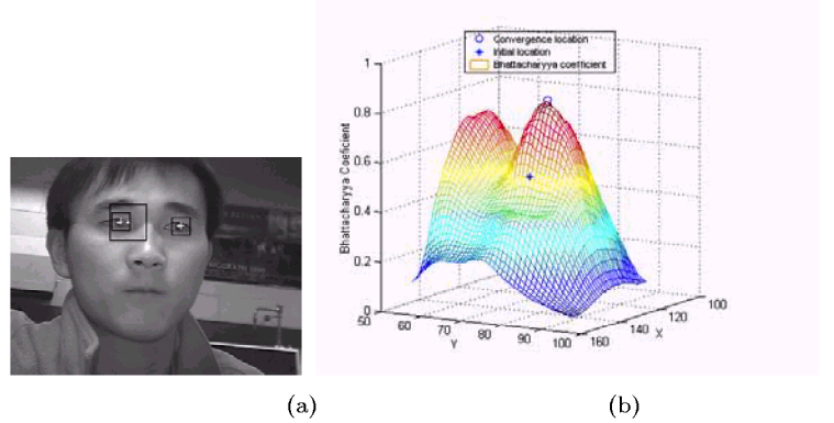
Figure 4. (a) The image frame 13; (b) Values of Bhattacharyya coefficient corresponding to the marked region ( 40 \times 40 pixels) around the left eye in frames 13. Mean shift algorithm converges from the initial location (*) to the convergence point (o) which is the mode of the surface.
