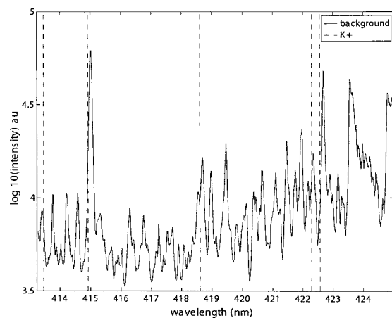
FIG. 4. Discharge averaged background plasma emission. The wavelengths at which we may expect to see emission from \text{K}^+ , when the beam is injected into the plasma, are shown as vertical dashed lines.
