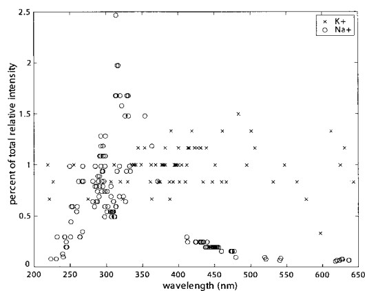
FIG. 3. Normalized \text{Na}^+ and \text{K}^+ emission intensities.
