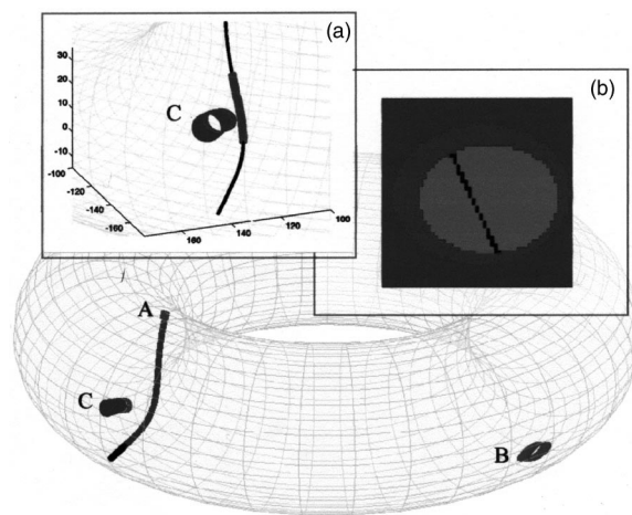
FIG. 2. (Color online) PerSpect simulation. (a) Enhanced segment of the trajectory is portion visible from end of wedge shaped chamber at port C. (b) The corresponding, simulated, CCD camera low-resolution image.
