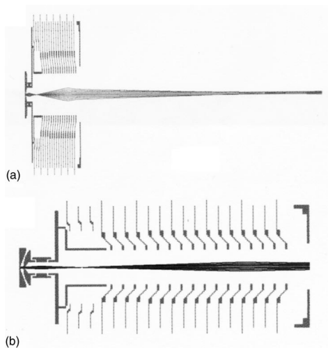
FIG. 1. (Color online) (a) Simulation of HIBP accelerator and ion beam (not to scale) that is well focused near the plasma. (b) Closeup of accelerator and beam. Beam is being focused by five rightmost column electrodes.
