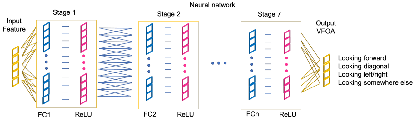
Figure 4: Details of the neural network architecture.
