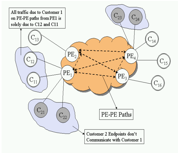
Fig. 6. Schematic indicating the structural aspects of VPNs that lead to additional equations in the Traffic Matrix estimation problem
