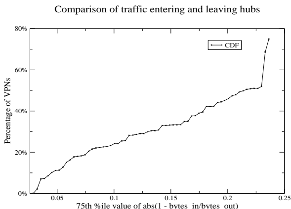
Fig. 12. CDF of 75 th %ile ratio of traffic entering a hub to the traffic leaving a hub for Hub/Spoke VPNs
