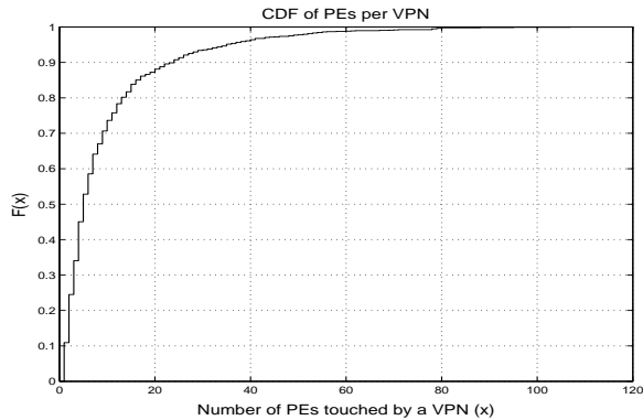
Fig. 3. CDF of number of PEs touched by a VPN
