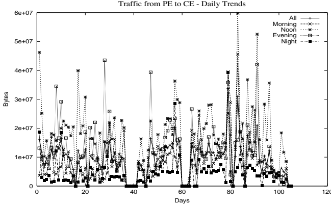
Fig. 5. Aggregate bytes entering a CE over 5 months for a VPN of size 79
