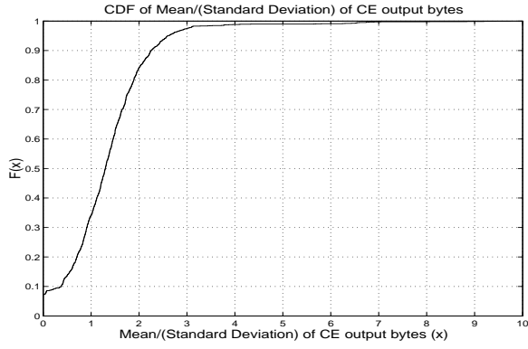
Fig. 7. CDF of the spread of spoke sizes from SNMP data for Hub/Spoke VPNs
