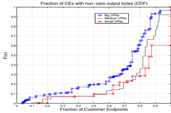
Fig. 10. CDF of fraction of CEs featuring non-zero output bytes confirms larger hub/spoke VPNs have more CEs with zero output bytes. This means that accuracy of estimates for larger Hub/Spoke VPNs is better.
