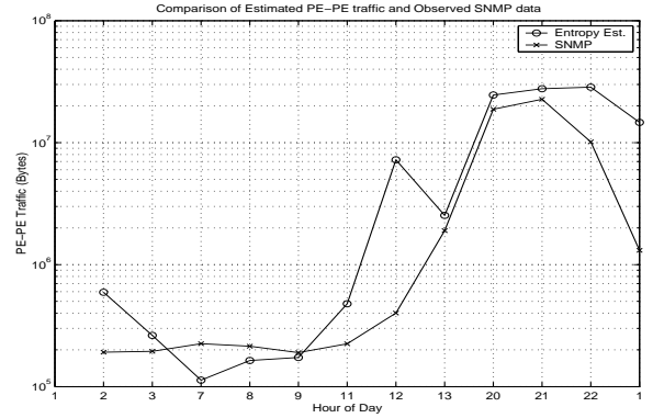
Fig. 16. Estimated traffic vs Observed traffic for a PE-PE link with lower traffic volume
