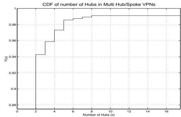
Fig. 13. CDF of number of hubs in multi-hub VPNs
