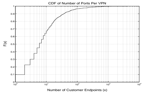
Fig. 4. CDF of number of CEs per VPN
