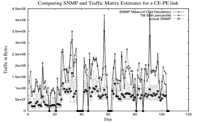
Fig. 15. Comparison of estimated CE output bytes with that derived from SNMP
