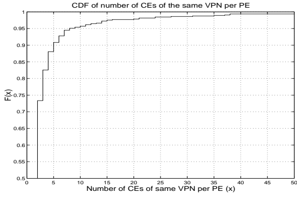
Fig. 14. CDF of number of CEs of the same VPN on a given PE
