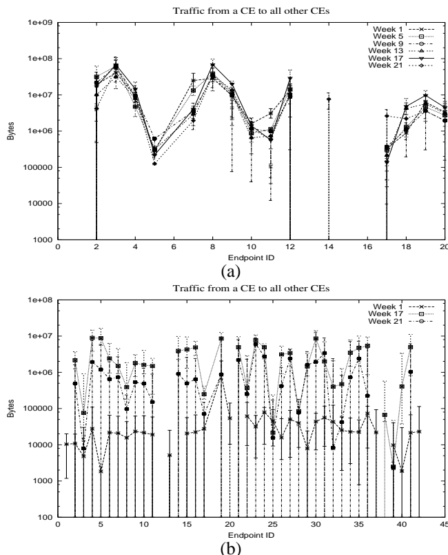
Fig. 27. Long term trends for traffic from a CE to all other CEs in VPNs of higher size
