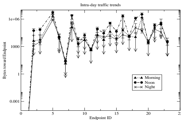
Fig. 25. An Endpoint communicating with multiple peers; traffic proportions to other endpoints are very similar for different times of day, although the magnitude varies.
