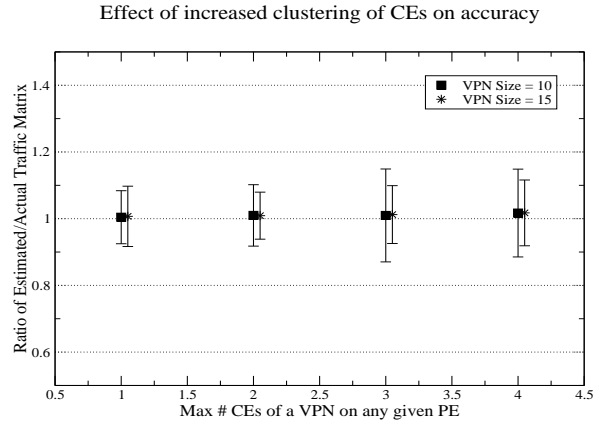
Fig. 8. Error in estimated traffic matrix increases with increased clustering of a customer’s endpoints on a PE
