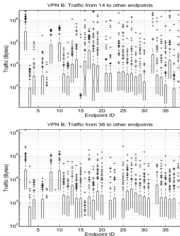
Fig. 24. A larger VPN exhibiting complex interactions between various endpoints. There are orders of magnitude difference in the amount of traffic toward different CEs
