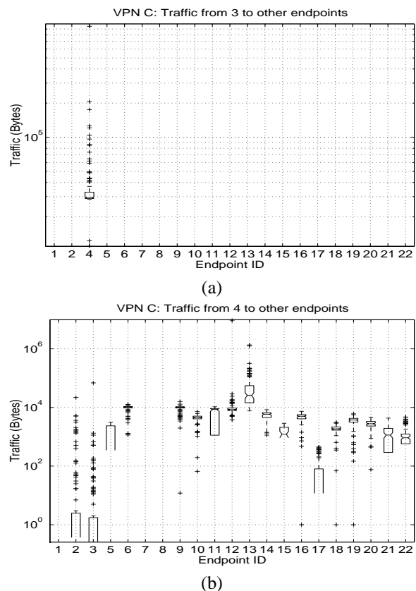
Fig. 23. Hub/Spoke-like behavior can be seen with some endpoints in VPNs such as above
