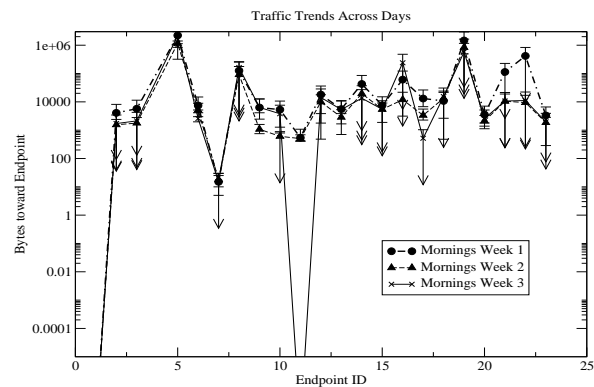
Fig. 26. Traffic trend from an endpoint to others in a VPN remains similar across multiple days.
