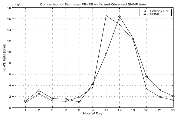
Fig. 17. Estimated traffic vs Observed traffic for a PE-PE link with higher traffic features better accuracy; estimates mimic the shape and order of the actual traffic in all cases
