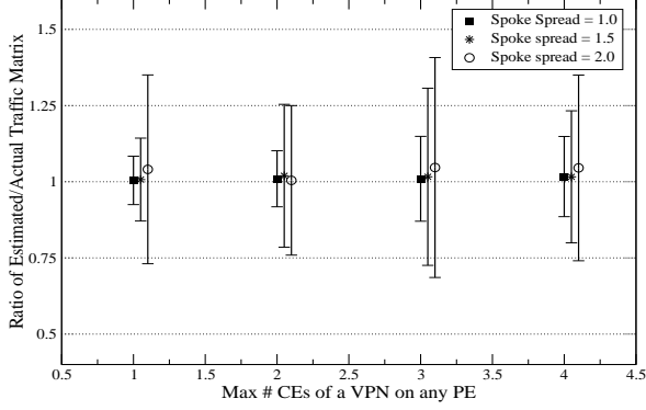
Fig. 9. Effect of cluster size with varying spread in spoke sizes for VPN of size 10. Smaller VPNs are affected more by increase in spread in spoke size
