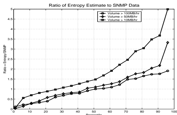
Fig. 18. The error decreases when we look at links with larger volume
