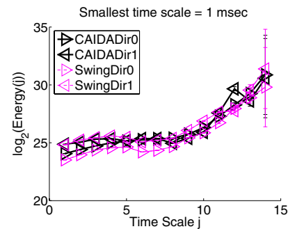
Figure 13: HTTP/CAIDA Energy plot (bytes).
