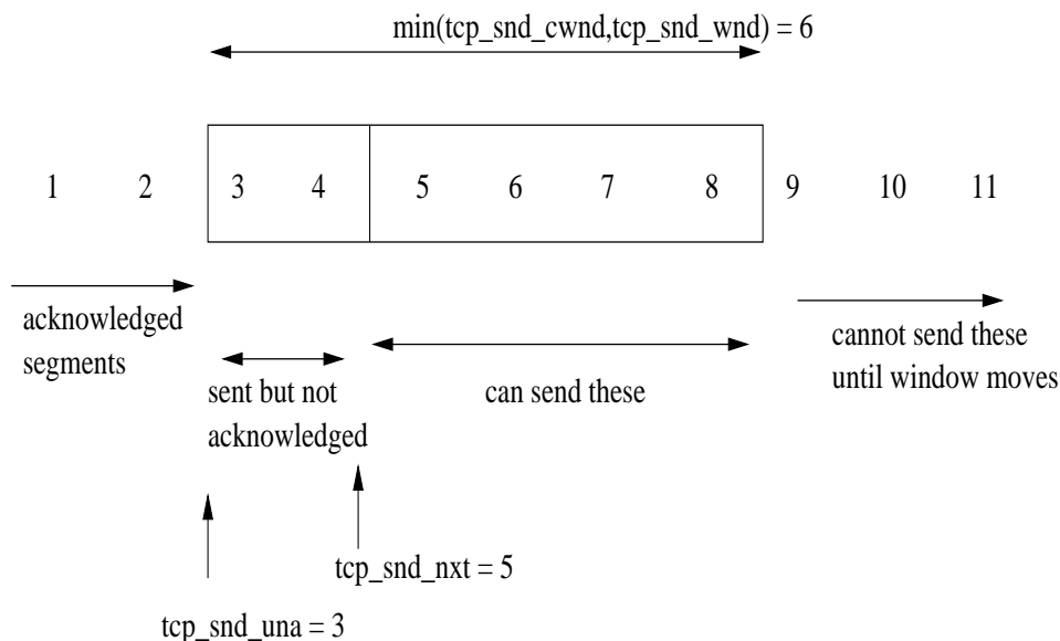
Figure 2: Sliding windows
