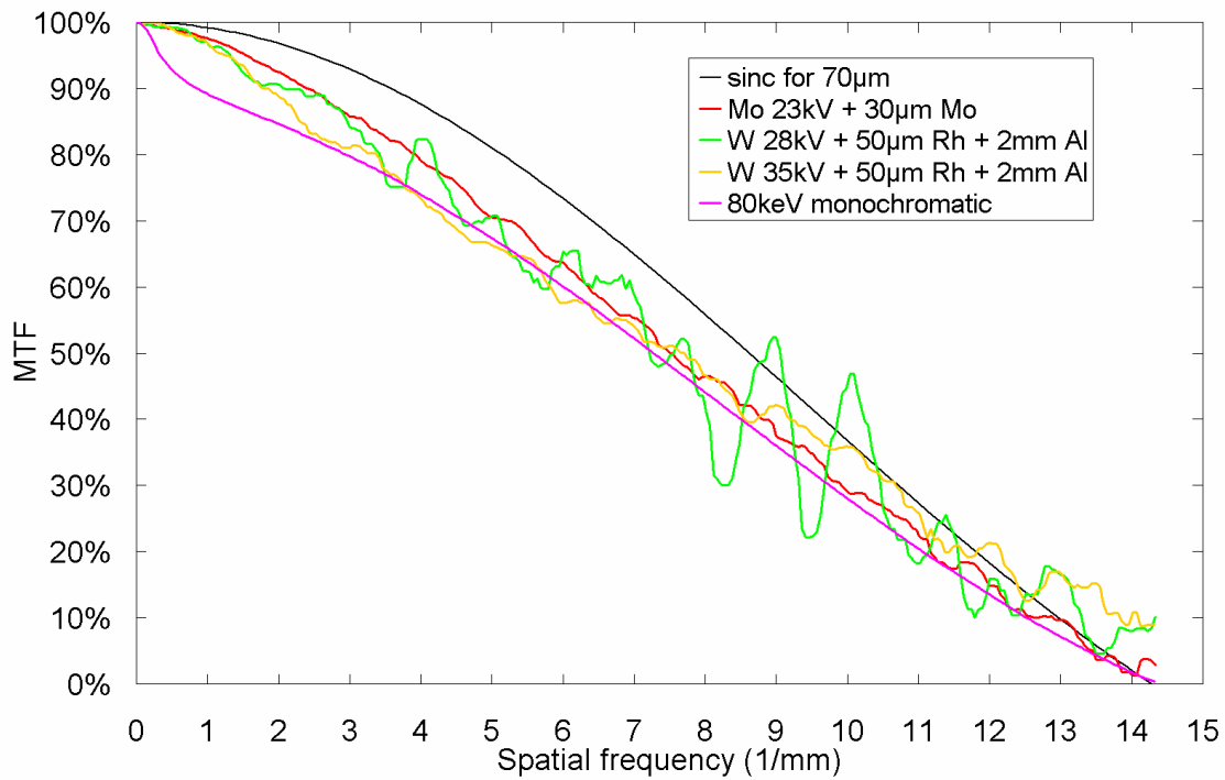
Fig. 7. Simulated MTF calculated for different mammography spectra. At higher energy (80 keV) a low-frequency drop due to backscattering from the substrate is visible.
