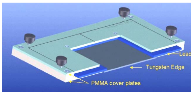
Fig. 1. A 2 mm thick tungsten edge phantom produced by Scanditronix / Wellhöfer.
