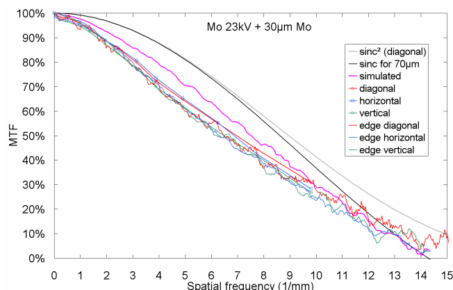
Fig. 3. MTF as a function of spatial frequency determined with a low energy mammography spectrum (Mo anode, 23 kV, 30 \mu\text{m} Mo prefiltration). Edge and lead bar method lead to comparable results. Furthermore, horizontal and vertical MTF are equal. The diagonal MTF is slightly higher, as is the theoretical limit, i.e. (2) instead of (1).
