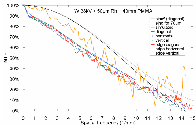
Fig. 6. MTF determined with a mammography spectrum (W anode, 28 kV, 50 \mu\text{m} Rh prefiltration, 40 mm PMMA additional filter). The low-frequency drop is around 10%.
