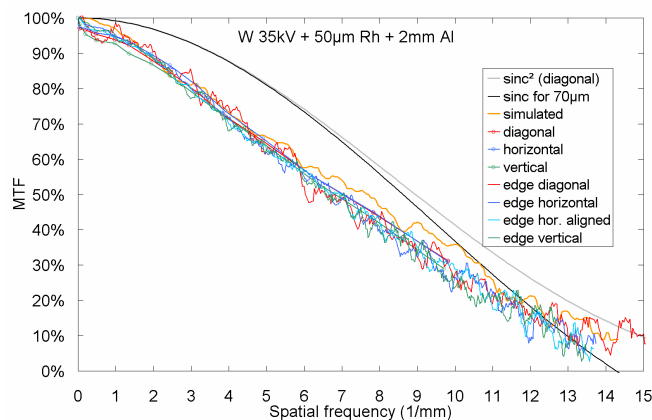
Fig. 4. MTF determined with a mammography spectrum (W anode, 35 kV, 50 \mu\text{m} Rh prefiltration, 2 mm Al additional filter). The edge positioned flat on the detector or aligned to the focus leads to equivalent results. The simulated MTF well agrees with the measurements.
