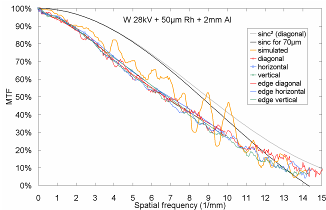
Fig. 5. MTF determined with a mammography spectrum (W anode, 28 kV, 50 \mu\text{m} Rh prefiltration, 2 mm Al additional filter). The low-frequency drop is 2% to 3%.
