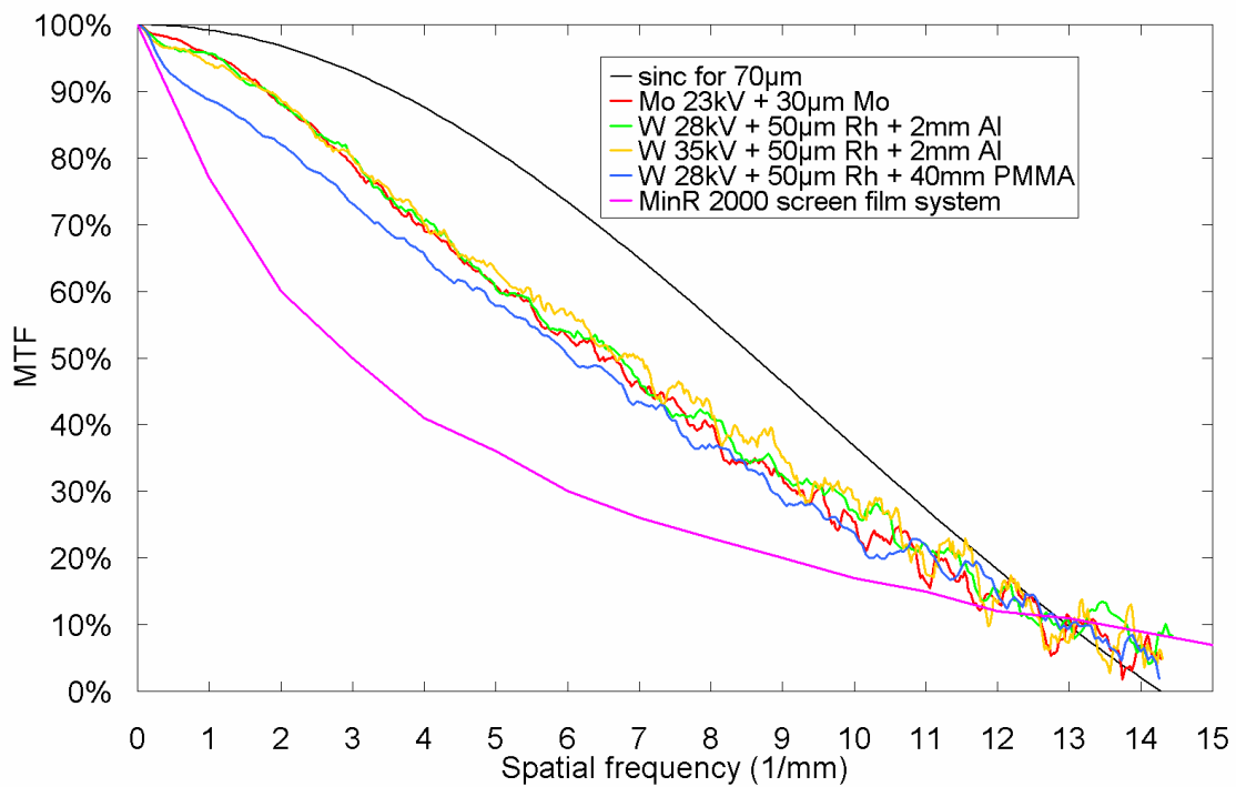
Fig. 8. Measured MTF for different mammographic spectra. PMMA filtering generates a low-frequency drop of around 10%. Data of a common film-screen system are given for comparison.
