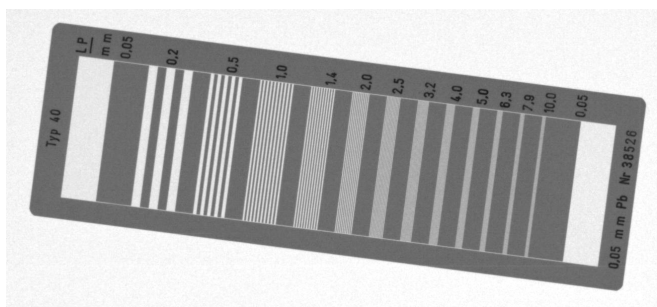
Fig. 2. Lead bar pattern type "40" produced by Hüttner. Spatial frequencies cover the range from 0.05 \text{mm}^{-1} to 10 \text{mm}^{-1} .
