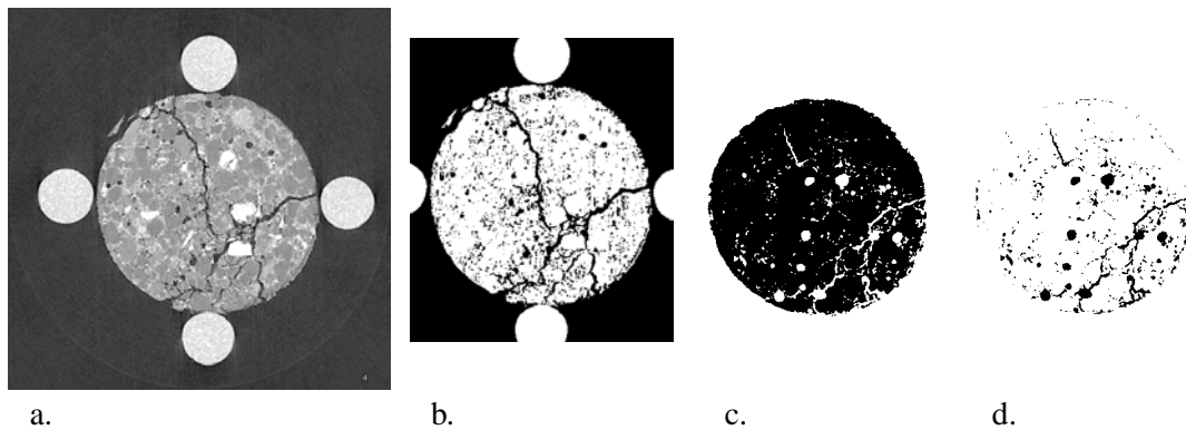
FIG. 1. Threshold-Based Procedure
