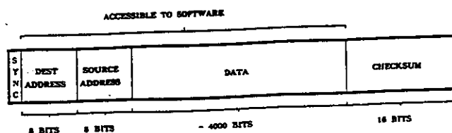
Fig. 2. Ethernet packet layout.
