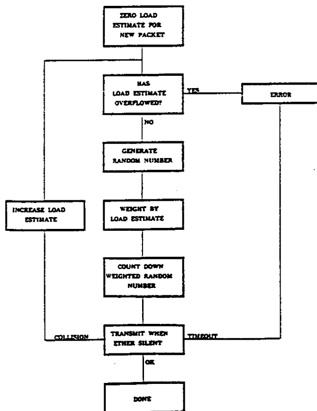
Fig. 3. Collision control algorithm.
