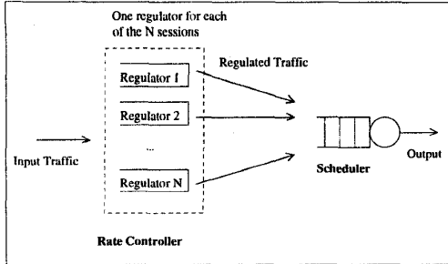
Figure 5: Rate-Controlled Service Discipline
