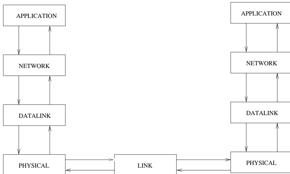
Figure 1: Layered Architecture
