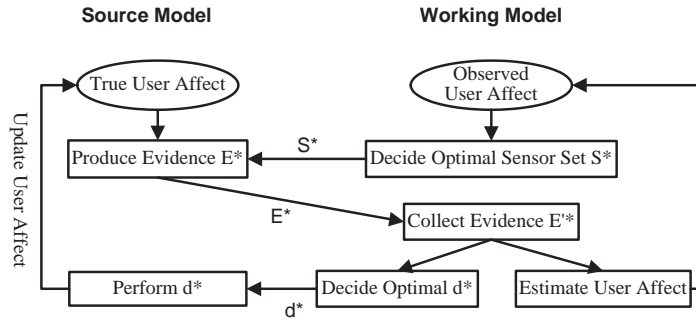
Fig. 10. A simulation system to validate the ID framework
