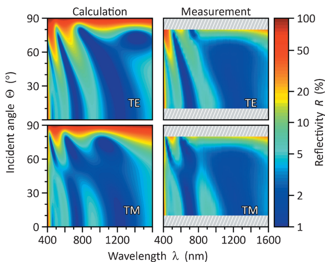
Fig. 4. Calculated and measured angle- and wavelength-averaged reflectivity of the four-layer AR coating on a silicon substrate.
