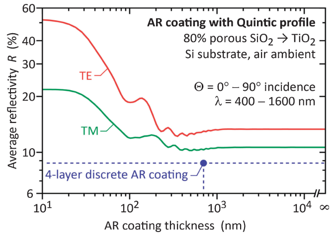
Fig. 2. Calculated angle- and wavelength-averaged reflectivity of an AR coating with a continuously graded quintic profile as a function of the coating thickness. Also shown is the averaged reflectivity of a discrete four-layer AR coating with thickness of approximately 700 nm. The discrete multilayer coating outperforms the continuously graded quintic profile for any thickness of the quintic coating.
