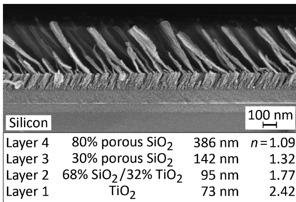
Fig. 3. SEM image of the four-layer AR coating on a silicon substrate, shown with layer composition, thickness, and refractive index data. The refractive index is given at a wavelength of 485 nm.
